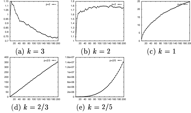
Fig. 1. |D_{max} - D_{min}| depending on d for different metrics (uniform data)
