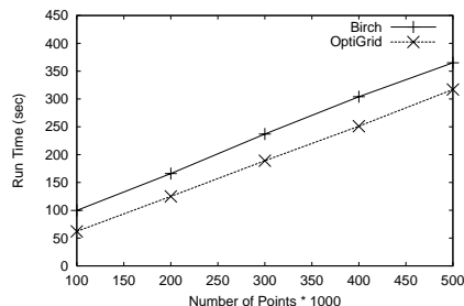
Figure 13: Performance Comparison
